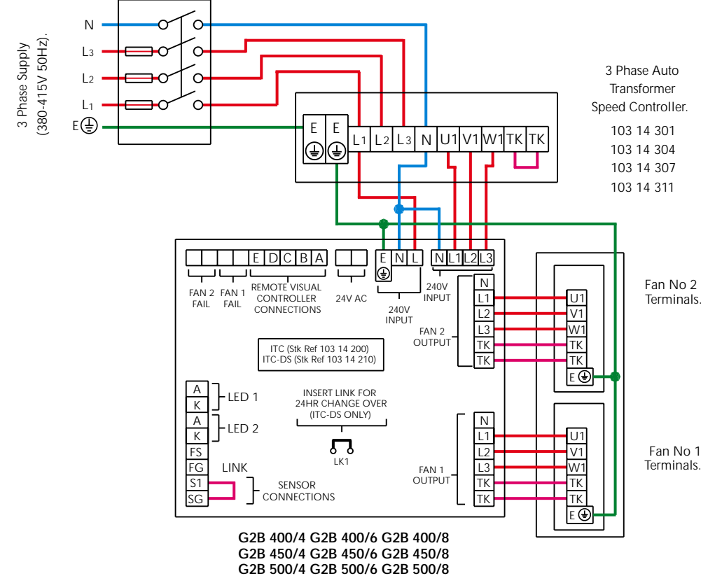
THREE PHASE FAN CONNECTED TO AN ITC CONTROLLER, AND AN AUTO TRANSFORMER CONTROLLER
